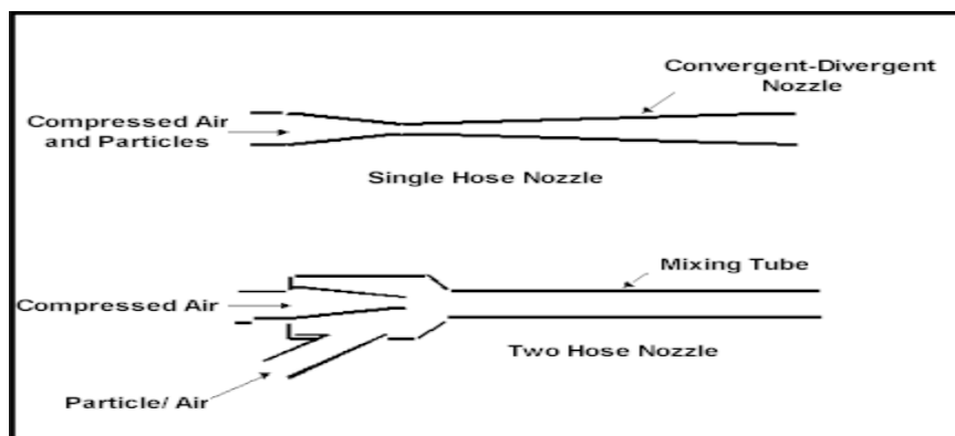
Figure 1 CO 2 / Dry Ice Blasting Nozzle Types
