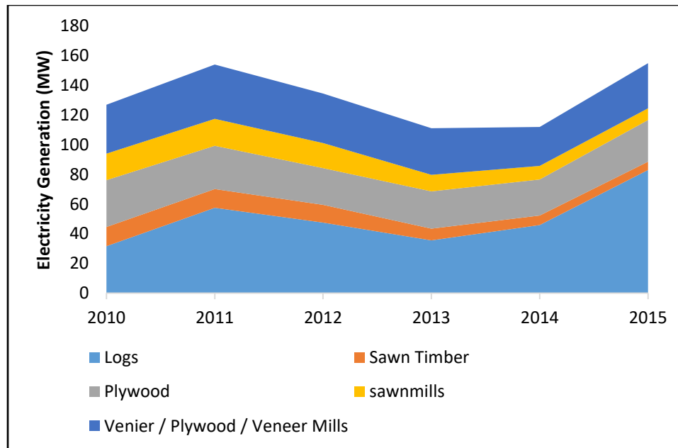
Figure 5 Potential electricity generation from wood residue in Kedah
